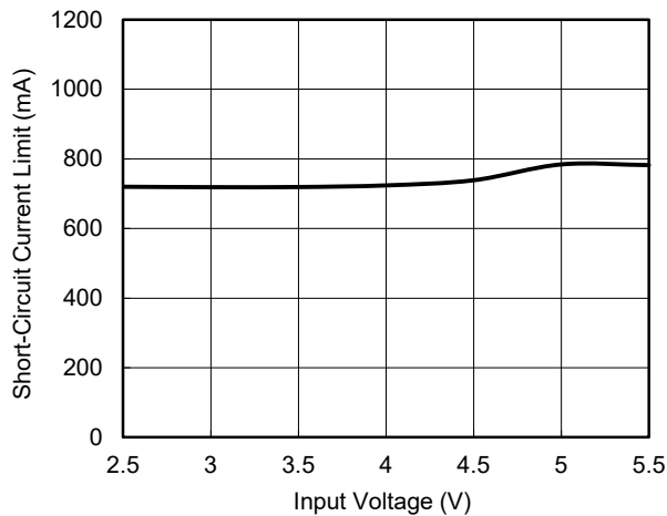
Short-Circuit Current Limit vs. Input Voltage (SGM2588A/B/G)
